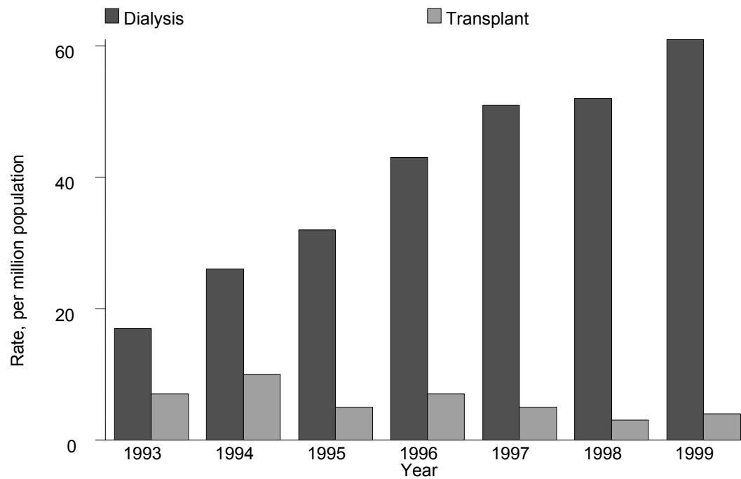
Figure 1.02 New Dialysis Acceptance and New Transplant Rate 1993 - 1999
