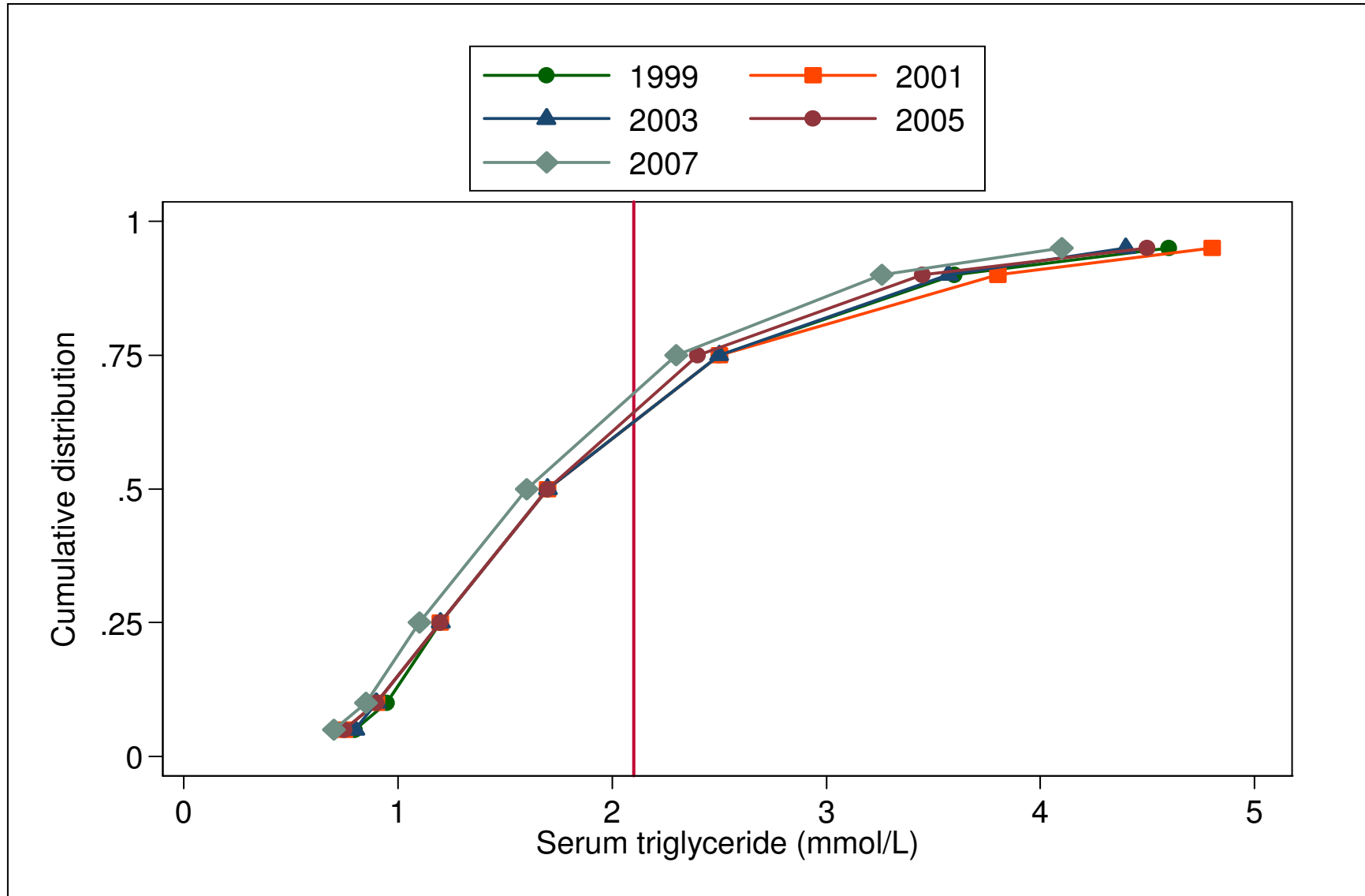
Figure 9.2.3: Cumulative distribution of serum triglyceride, HD patients 1998-2007
